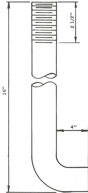
3/4" \phi ANCHOR BOLT X 16" LONG
